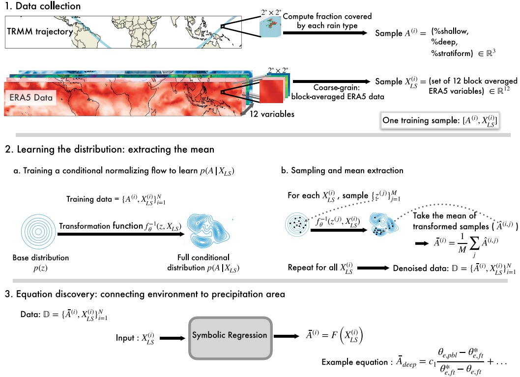
FIG. 1. A schematic summarizing our methods going from observations to equations. 1) Data collection. TRMM precipitation swaths are intersected with 2^\circ \times 2^\circ boxes. Within each box, we compute the fractional area covered by shallow, deep, and stratiform rain, forming a target vector A^{(i)} \in \mathbb{R}^3 . In parallel, ERA5 fields are coarse grained to the same blocks and reduced to 12 large-scale variables, yielding a conditioning vector X_{LS}^{(i)} \in \mathbb{R}^{12} . Each training example is a pair (A^{(i)}, X_{LS}^{(i)}) . 2) Learning the distribution and extracting the mean. A CNF learns the full conditional distribution p(\mathbf{A} | \mathbf{X}_{LS}) by transforming samples from a simple base density through a learned map f_\theta^{-1}(z, \mathbf{X}_{LS}) . For each \mathbf{X}_{LS}^{(i)} , we draw M noise samples, obtain \hat{\mathbf{A}}^{(i,j)} \sim p(\mathbf{A} | \mathbf{X}_{LS}^{(i)}) , and compute the conditional mean \bar{\mathbf{A}}^{(i)} = (1/M) \sum_{j=1}^M \hat{\mathbf{A}}^{(i,j)} . Repeating this for all i yields a noise-free dataset \{(\bar{\mathbf{A}}^{(i)}, \mathbf{X}_{LS}^{(i)})\}_{i=1}^N . 3) Equation discovery. The extracted pairs are used in symbolic regression to identify interpretable equations of the form \bar{\mathbf{A}} = F(\mathbf{X}_{LS}) , linking large-scale environment to mean precipitation area. For clarity, the distributions in step 2 are drawn in two dimensions; in practice, \mathbf{A} is three-dimensional and the flow learns a distribution in \mathbb{R}^3 .
