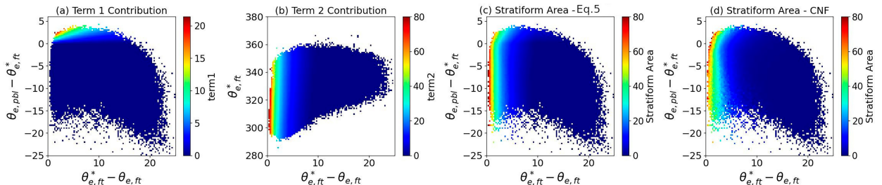
FIG. 7. As in Fig. 6, but for stratiform rain area following Eq. (5).
