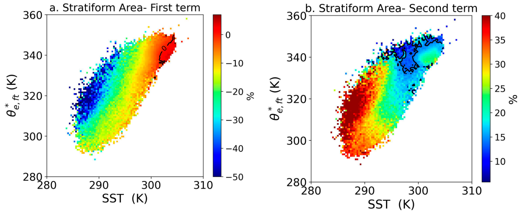
FIG. 9. Phase space structure of the two components that enter the stratiform-area closure [Eq. (5)]. (a) First (boundary layer buoyancy surplus) term; (b) second (FT deficit) term. Both panels are binned in SST ( x axis) vs FT saturated equivalent potential temperature, \theta_{e,ft}^* ( y axis). Color shading indicates the magnitude of each term as a percentage, and black contours trace the zero line where each trigger operator switches on.
