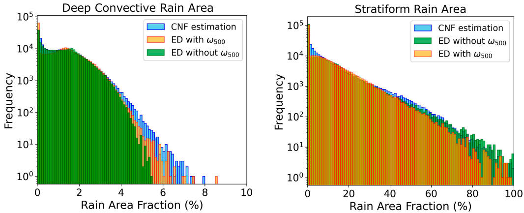
FIG. B1. Rain area distributions predicted by ED using CRH with and without \omega_{500} , compared against the CNF benchmark (blue). (left) Deep convective area, corresponding to the CRH-based equations with \omega_{500} [orange; Eq. (B1)] and without \omega_{500} [green; Eq. (B2)]. (right) Stratiform area, corresponding to the CRH-based equations with \omega_{500} [orange; Eq. (B3)] and without \omega_{500} [green; Eq. (B4)]. Including \omega_{500} yields substantially simpler equations that more accurately capture the tails of the distributions, while excluding it requires more complex expressions to approximate the same behavior.
