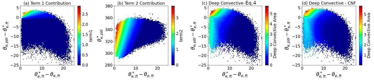
FIG. 6. Two-dimensional histograms illustrating the individual terms and overall performance of the deep convection closure, Eq. (4). All panels use the FT saturation deficit (K) on the x axis. The y axis shows the boundary layer buoyancy surplus (K) in (a), (c), and (d) and the saturation value \theta_{e,pbl}^* in (b), consistent with the variables appearing in each term of the equation. Each bin ( \Delta x = \Delta y = 0.3 K) aggregates all samples within it; color indicates the mean rain area per bin. (a) Contribution of the buoyancy-overdryness term, (b) contribution of the humidity gate, and deep convective area predicted (c) by Eq. (4) and (d) by the CNF.
