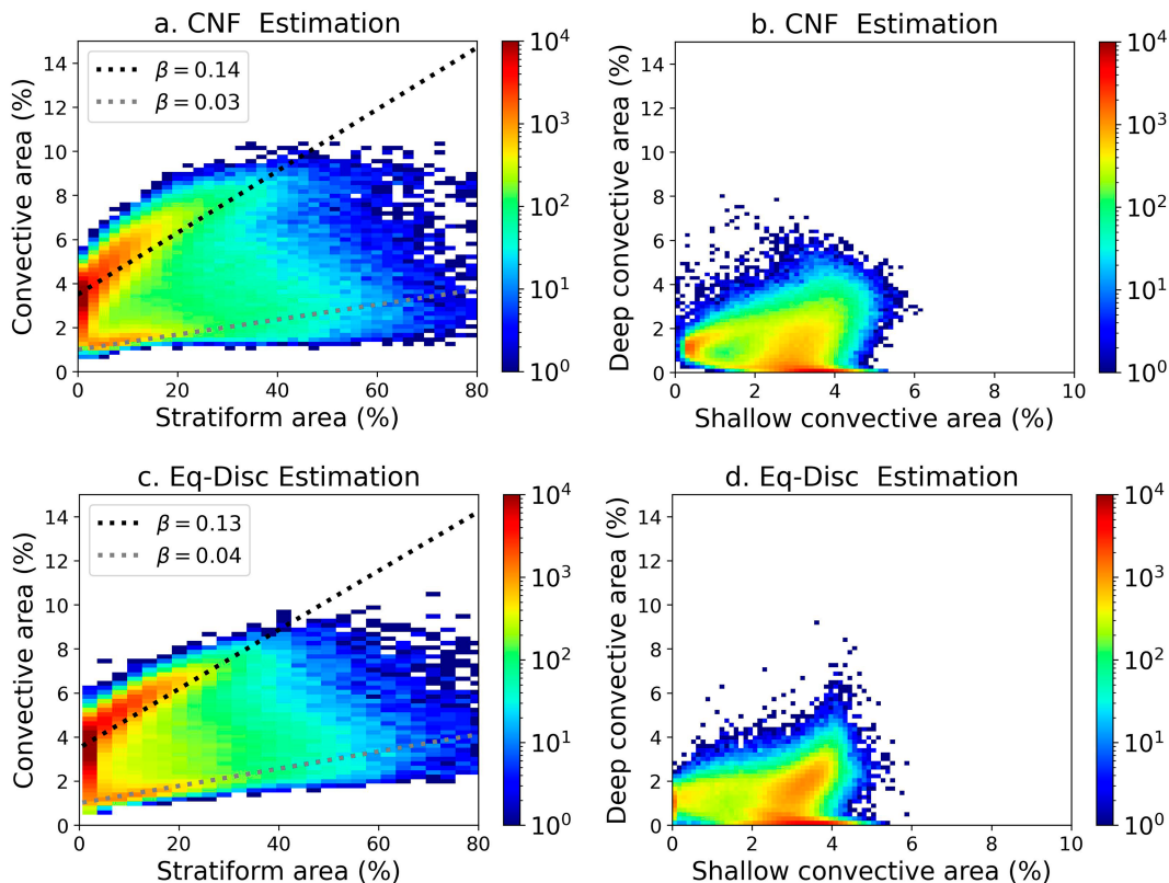
FIG. 4. Two-dimensional histograms of rain areas predicted by the CNF model (means) and by the equation discovery (Eq-Disc) model. (a),(c) Total convective area (deep + shallow) vs stratiform area; (b),(d) deep vs shallow convective area. Color indicates frequency on a logarithmic scale. In (a) and (c), the black and gray dotted lines represent linear regressions between total convective and stratiform areas, with the estimated slopes shown in the legend.
