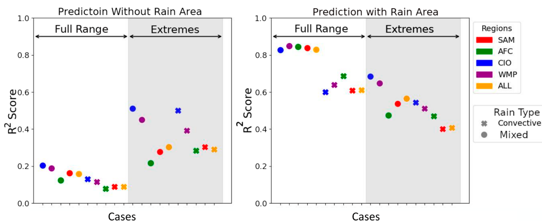
FIG. A1. Precipitation predictability with and without rain area information. The R^2 scores for predicting rain rate averaged over the grid box (left) without and (right) with rain area information as input. Each point represents a different region (indicated by color), and marker shapes distinguish precipitation types: “x” for convective only (including shallow and deep convective) and “o” for total precipitation (including shallow convective, deep convective, and stratiform). Shaded regions highlight predictions for extreme precipitation events; unshaded areas represent predictions over the full distribution of precipitation amounts.
