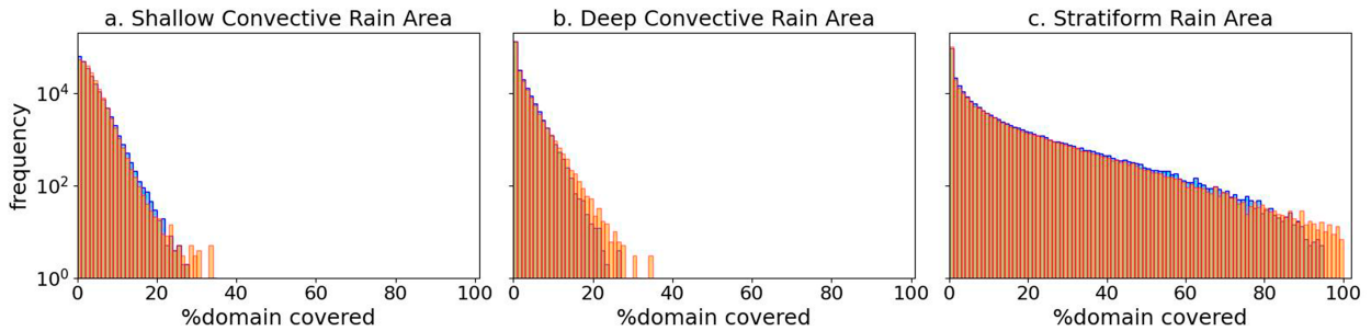
FIG. 2. Marginal distribution of (a) shallow convective, (b) deep convective, and (c) stratiform rain areas. Blue indicates observed data, and orange represents the CNF generated distribution.
