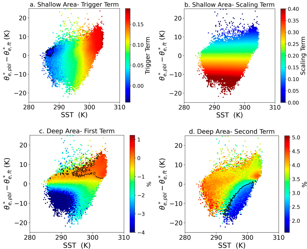
FIG. 8. Figure shows sensitivity of convective rain areas to surface temperature and atmospheric stability. All subplots share the same axes: x axis is SST (K); y axis is \Delta\theta^* = \theta_{e,pbl}^* - \theta_{e,ft}^* (K). Points are 2D bins colored by the mean value of the indicated analytic term; higher (warmer) colors denote larger positive values. A solid black contour marks the zero line of the corresponding trigger operator, i.e., where the term switches from inactive to active. (a) Shallow convection trigger term [Eq. (3); second bracket]. (b) Shallow convection scaling term [always-positive prefactor in Eq. (3)]. (c) Deep convection buoyancy–dryness term [first term in Eq. (4)]. (d) Deep convection humidity gate [second term in Eq. (4)].
