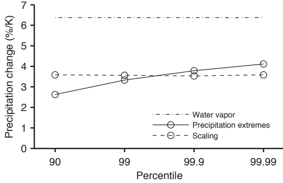
FIGURE 5: Fractional rates of increase with global-mean surface temperature at the reference simulation for the global-mean precipitation extremes (solid), precipitation extremes scaling (4) (dashed), and water vapor content (dash-dotted). Values are shown for the 90th, 99th, 99.9th, and 99.99th percentiles. The rates of increase in the precipitation extremes are 2.6, 3.3, 3.8, and 4.1%/K. The rates of increase in the scaling are 3.6, 3.6, 3.5, and 3.6%/K. The rate of increase in the water vapor content is 6.4%/K.
