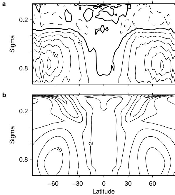
FIGURE 7: (a) Temperature difference T_e - \bar{T} between the temperature corresponding to the 99.9th percentile of precipitation and the mean temperature for the reference simulation. Positive values indicate that it is warmer than average when the extreme precipitation occurs. (b) 1.7 T_{rms} corresponding to the approximation (5). Positive contours are solid, negative contours are dashed, and the zero contour is shown with a thicker line. The contour interval is 2 K.
