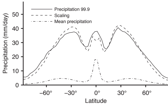
FIGURE 1: 99.9th percentile of daily precipitation (solid) and mean precipitation (dash-dotted) in the reference simulation ( \alpha = 1 ). The precipitation extremes scaling (4) is also shown (dashed), multiplied by a constant of proportionality of 3.5 so that it agrees with the 99.9th percentile in the global mean. Statistics shown here and in the following figures are based on zonal and time averages. Deviations from symmetry between the hemispheres are indicative of sampling error.
