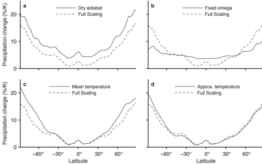
FIGURE 8: Simplified variations of the precipitation extremes scaling (4) for the 99.9th percentile precipitation. Dashed lines show the full scaling. Solid lines: (a) Not accounting for changes in the moist-adiabatic lapse rate by using the dry-adiabatic lapse rate in (2) to calculate dq_s/dp|_{\theta^*} . (b) Holding \omega_{rms} fixed at its reference simulation values. (c) Using mean temperature instead of the temperature of the precipitation extremes T_e . (d) Using the approximation T_e = \bar{T} + 1.7 T_{rms} . Values shown are fractional changes between the reference simulation ( \alpha = 1 ) and a warmer simulation ( \alpha = 1.4 ), expressed relative to the reference simulation values and normalized by the change in global-mean surface temperature (compare with Fig. 2). The changes shown have been smoothed in latitude with a 1-2-1 filter.
