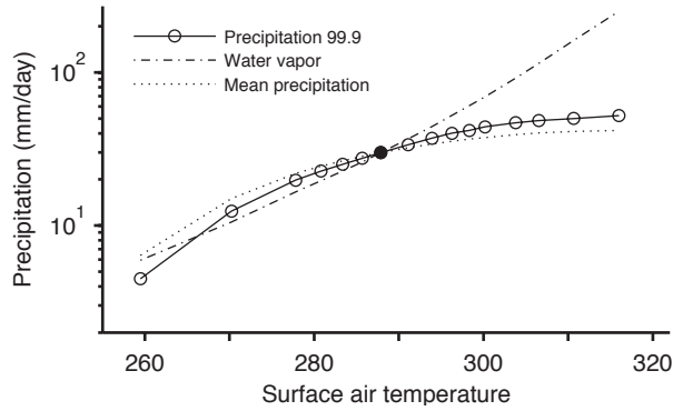
FIGURE 3: Global-mean of the 99.9th percentile precipitation rate vs global-mean surface temperature (solid line with circles) shown on a log-linear plot. The reference simulation is shown with a filled circle. Also shown is the rescaled global-mean water vapor content (dash-dotted) and the rescaled global-mean precipitation (dotted). Both the water vapor content and mean precipitation curves have been rescaled by dimensional constants so that they can be compared with the extreme precipitation and coincide with it at the reference simulation. At the reference simulation, the fractional rate of increase with global-mean surface temperature is 6.4%/K for water vapor content, 3.8%/K for the 99.9th percentile of precipitation, and 2.5%/K for mean precipitation.
