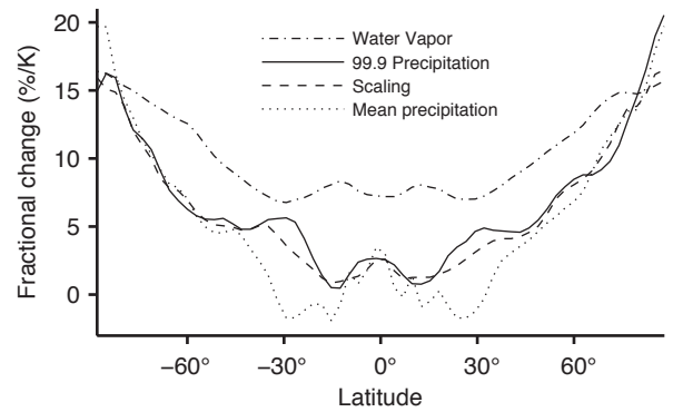
FIGURE 2: Fractional changes between the reference simulation ( \alpha = 1 ) and a warmer simulation ( \alpha = 1.4 ) expressed as a percentage of the reference simulation values: column water vapor (dash-dotted), 99.9th percentile of daily precipitation (solid), precipitation extremes scaling (4) (dashed), and mean precipitation (dotted). The changes are normalized by the global-mean surface temperature difference of 6.1 K between the two simulations. The changes shown for the 99.9th percentile precipitation and the scaling have been smoothed in latitude with a 1-2-1 filter.
