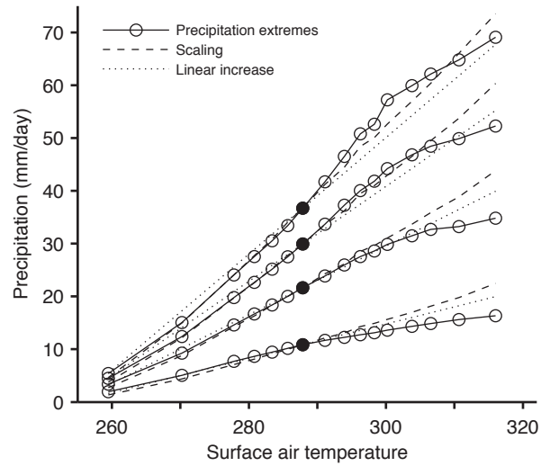
FIGURE 4: Global-mean of high percentiles of precipitation rate vs global-mean surface temperature (solid lines with circles). The reference simulation is shown with filled circles. The percentiles shown are the 90th, 99th, 99.9th, and 99.99th, in increasing order of precipitation rate. The precipitation extremes scaling (4) is shown with a dashed line for each percentile and has been normalized in each case to pass through the reference simulation value (rescaling constants of 1.3, 2.6, 3.5, and 4.2). The dotted lines show linear increases at 3%/K relative to the reference simulation.
