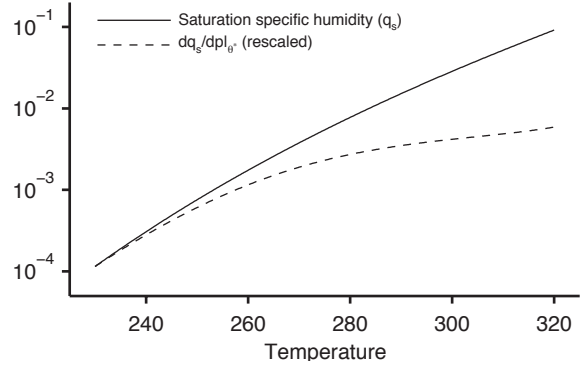
FIGURE 6: Saturation specific humidity (solid) and the rescaled moist-adiabatic derivative of saturation specific humidity dq_s/dp|_{\theta^*} (dashed). Both quantities are evaluated at a pressure of 800 hPa. The moist-adiabatic derivative of saturation specific humidity has been rescaled by a dimensional constant so that it agrees with the saturation specific humidity at the lowest temperature shown. At 280 K, the fractional rate of increase in saturation specific humidity is 6.9%/K, compared with 3.0%/K for the moist-adiabatic derivative of saturation specific humidity.
